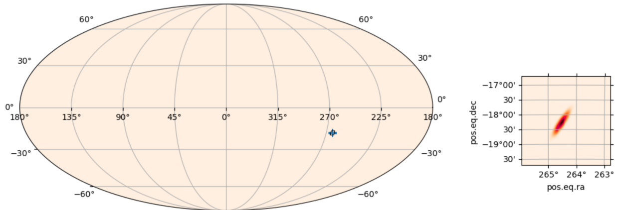
FIGURE 4: The injected localization skymap for 3I/ATLAS ToO observations on the night of July 12, 2025.
